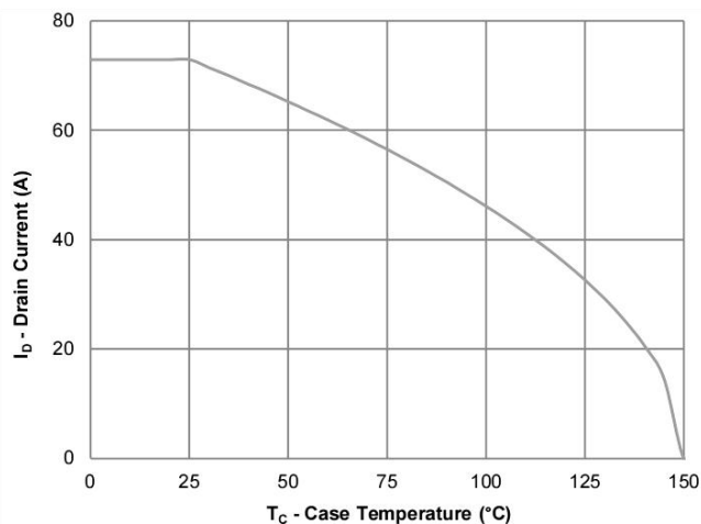
Figure 11: Current Derating
