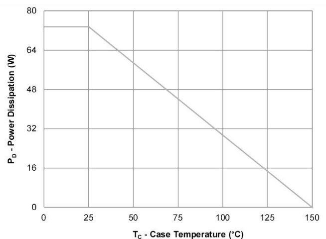
Figure 10: Power Derating
