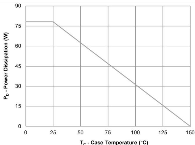
Figure 10: Power Derating
